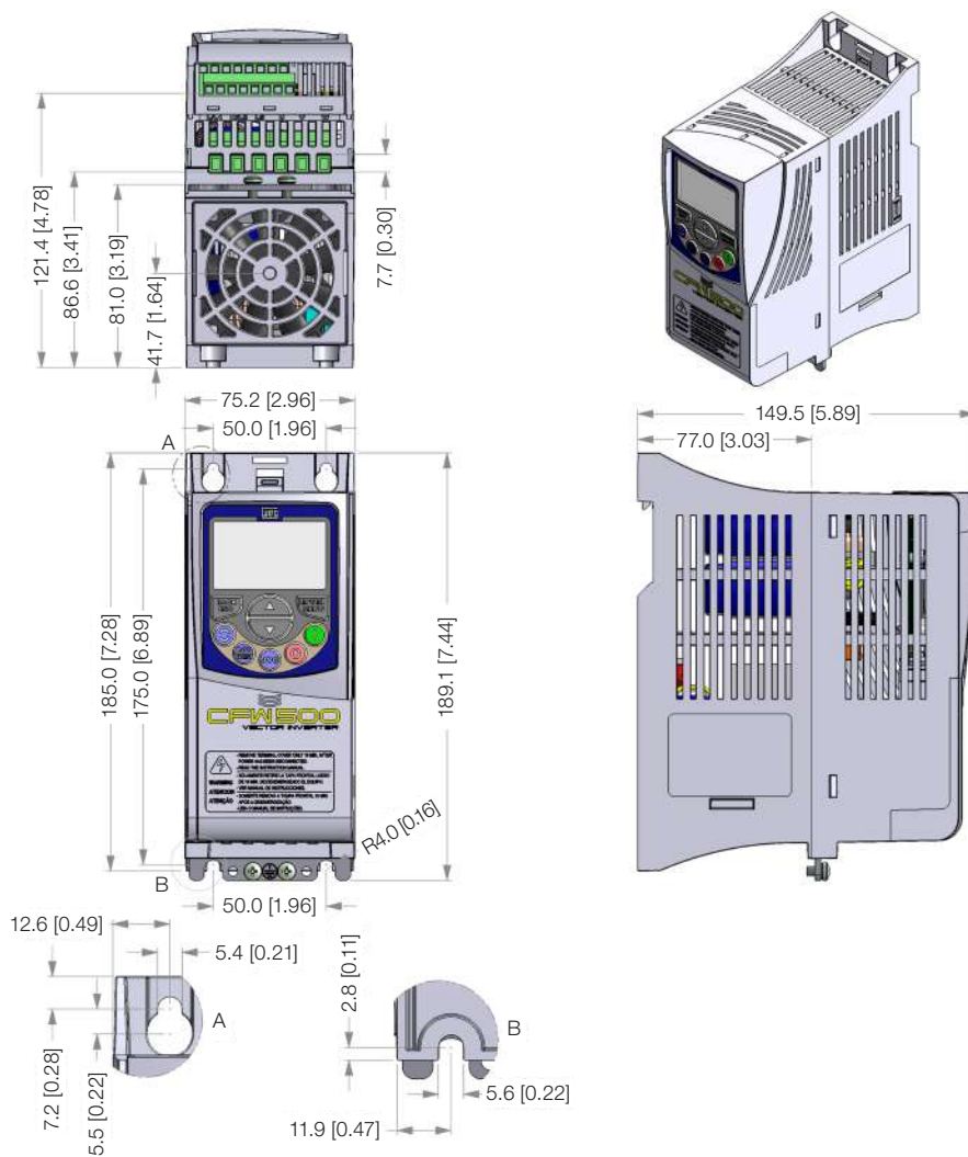
Figure B.5: Inverter dimensions in mm [in] - frame size A
